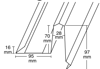
Barge Soaker
