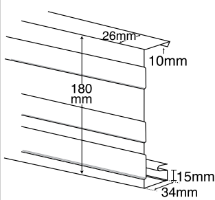
Steel Fascia
