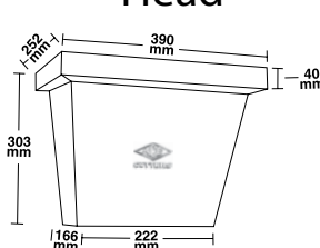
Rainwater Head
