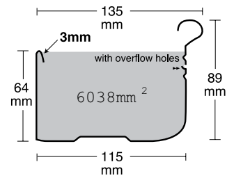
Fascia Cover
