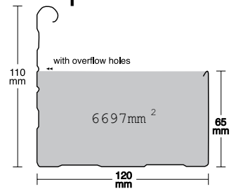
Barge Soaker
