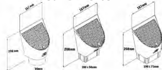
Concealed
