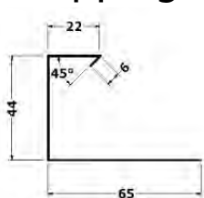
Capping
