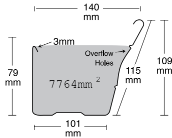
Roundline Slotted
