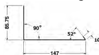
Soaker Flashing
