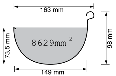
Valley
