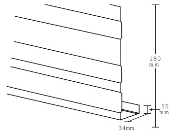
Square-Line
